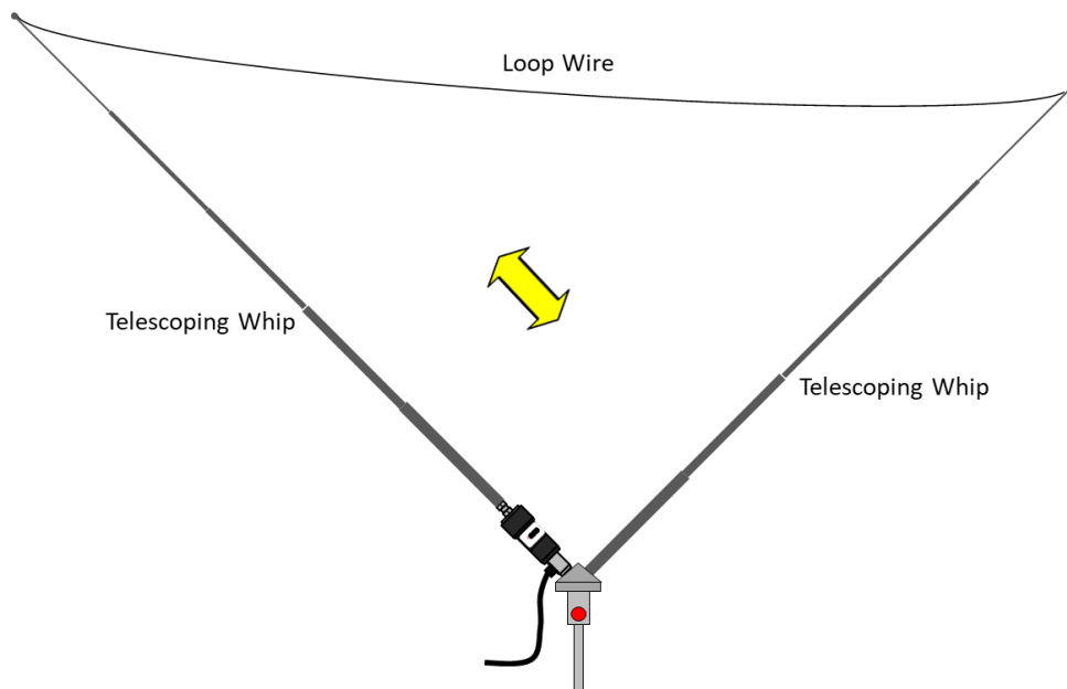
Figure 1. Inverted Delta Loop Configurations.
