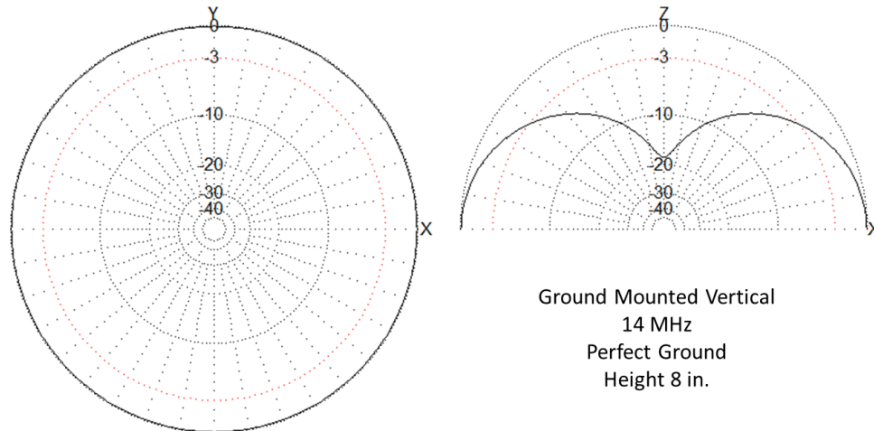
Figure 5. Ground Mounted Vertical Far Field Plot.
