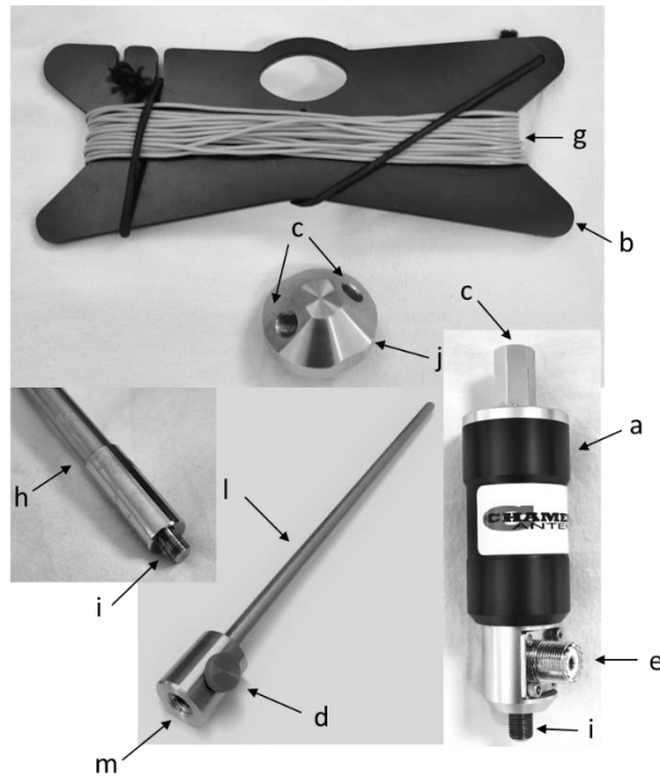
Plate 2. Tactical Delta Loop Components.
