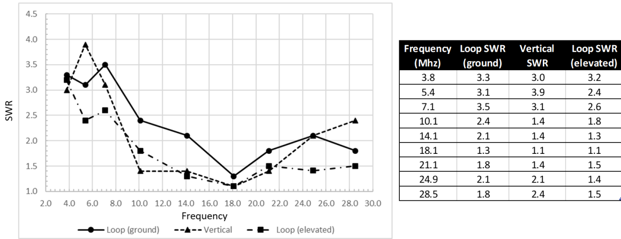
Figure 3. Typical Tactical Delta Loop Measured SWR.
