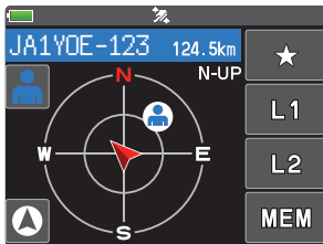
Backtrack Screen
