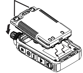
Battery Latches
