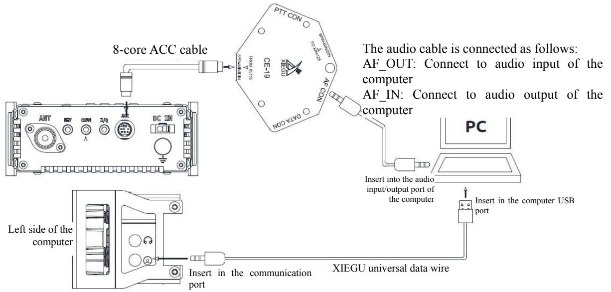
Fig. 1 G90 and Computer Connection Data Communication Diagram
