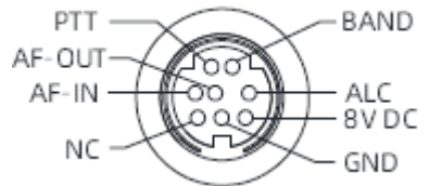
Tail ACC socket
