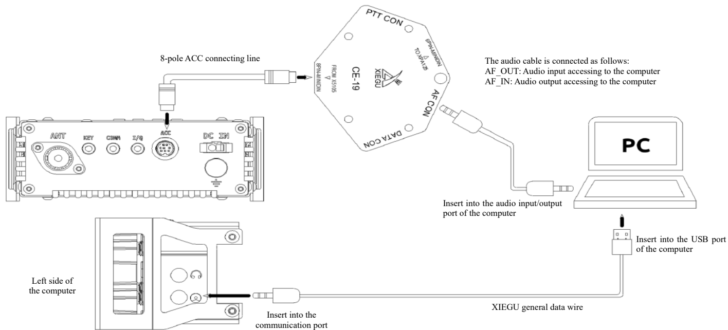
Schematic Diagram of Connection between CE-19 and G90S
