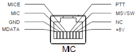
Microphone port
