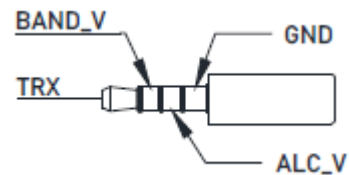
Definition of ACC interface
